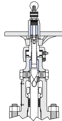
OS&Y Packing
